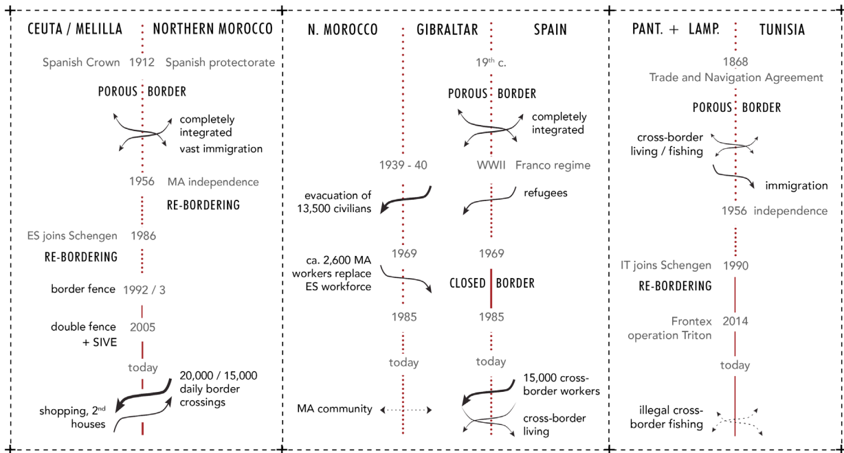
FIG. 2 CIs' border enforcement and transcendence in the past century. Source: author's elaboration based on the cited literature.
